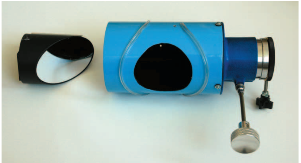
Housed in a short length of tubing is the refractor's "bending mirror" — a Newtonian-reflector diagonal that directs light from the objective lens to a star diagonal (not shown) inserted into the focuser.
